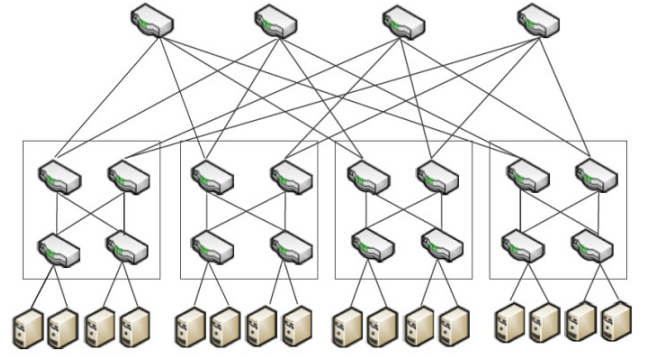
Fig. 2. Fat-tree data center network with four ports
