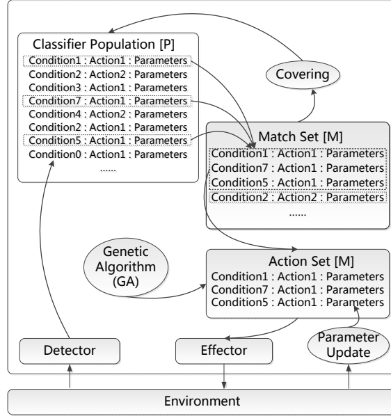
Figure 1. XCS framework
