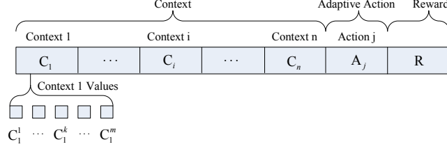
Figure 3. Training rule
