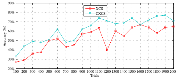
Figure 7. Training accuracy using cooperative cover and predicting
