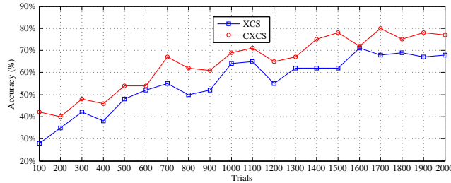
Figure 6. Training accuracy using cooperative initialization
